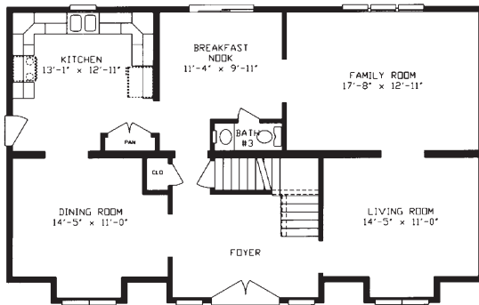
FIRST FLOOR 2376 SQ. FT.
