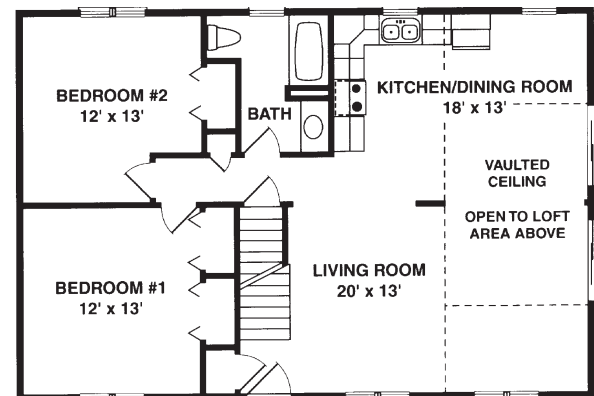
FIRST FLOOR 1120 SQ. FT.
