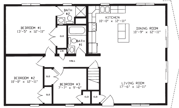
TIMBERLAKE 1232 SQ. FT.
